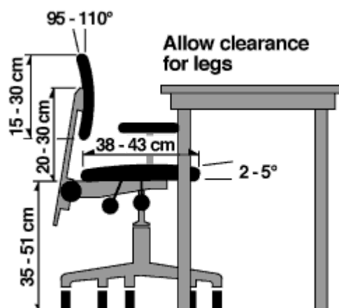
Ergonomic Chair
